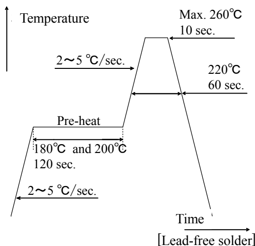
■ Temperature profile
