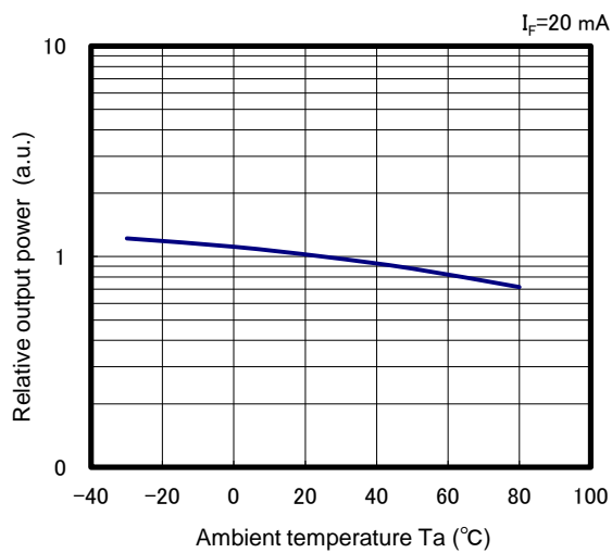
■ Ambient temperature vs. Relative output power
