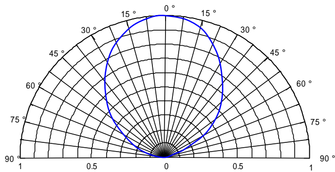
Directivity
